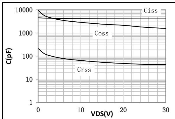
Fig.2 Capacitance Characteristics
